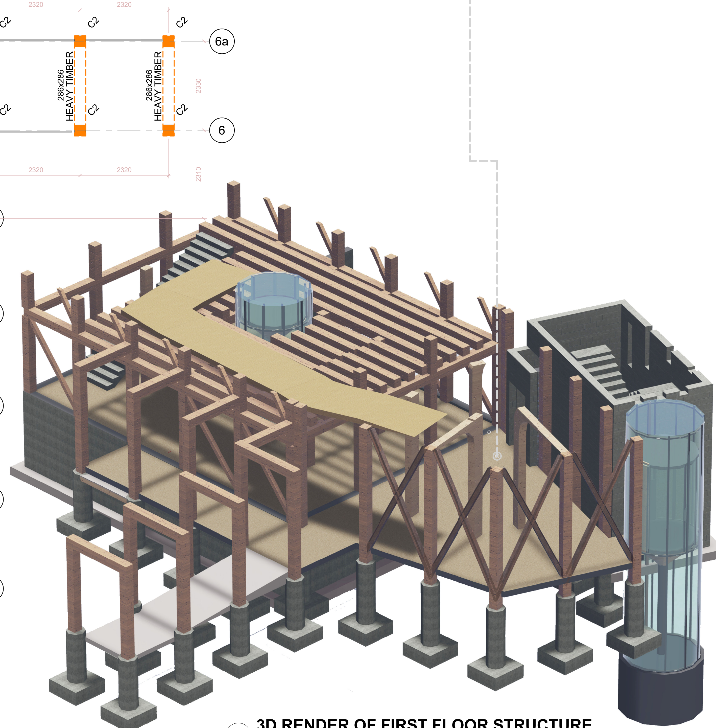
2 3D RENDER OF FIRST FLOOR STRUCTURE
