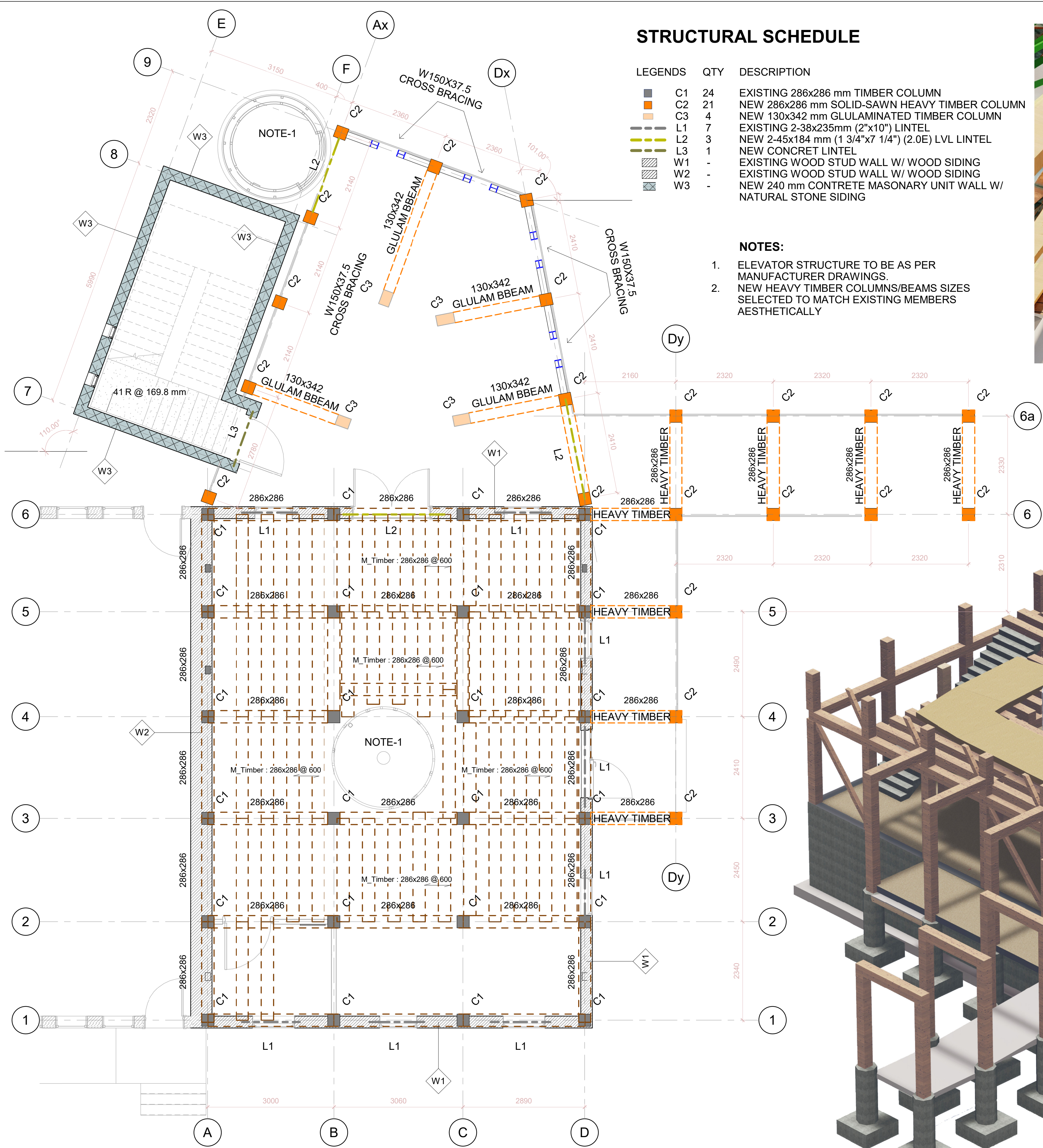
1 FIRST FLOOR STRUCTURAL PLAN 1 : 50
